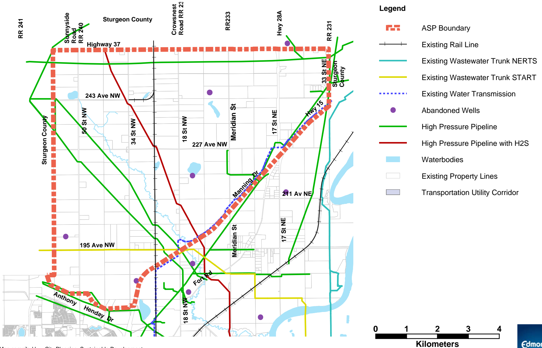
Figure 5: Existing Pipelines and Wells
